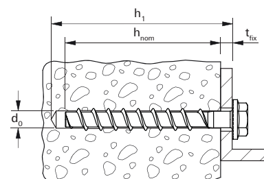
ULTRACUT FBS II US - hexagon head with pressed washer
